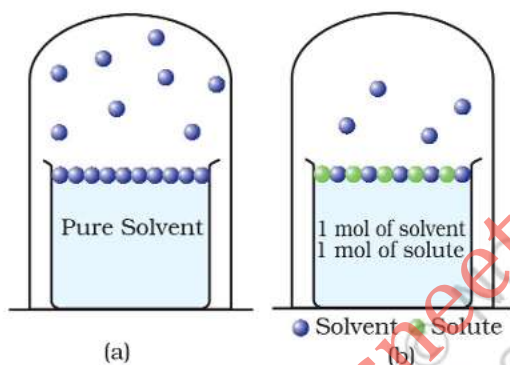
Fig. 2.4: Decrease in the vapour pressure of the solvent on account of the presence of solute in the solvent (a) evaporation of the molecules of the solvent from its surface is denoted by \bullet , (b) in a solution, solute particles have been denoted by \bullet and they also occupy part of the surface area.
